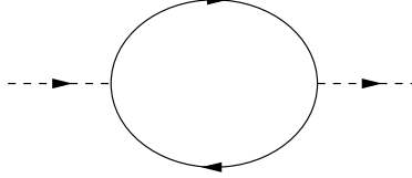
FIG. 1. Shows the quadratic term resulting from the expansion in small e\phi . Solid lines represent a fermion loop and the dashed lines represent the gauge parameter. Associated with each vertex is the factor -ie\gamma^0\delta(t) .
